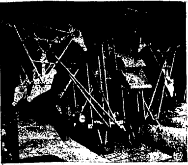
Their queer-looking, wingless "plane" almost ready for a test, Henri Van Zandt and Louis Chequet, French inventors working at Fort Chester, N. Y., confidently expect the contrivance, pictured above, to rise vertically into the air and remain virtually motionless if the pilot desires. The ferris-wheel-like contraptions jutting from all sides are telescopic blades intended to lift it aloft by "scooping" up the air.
