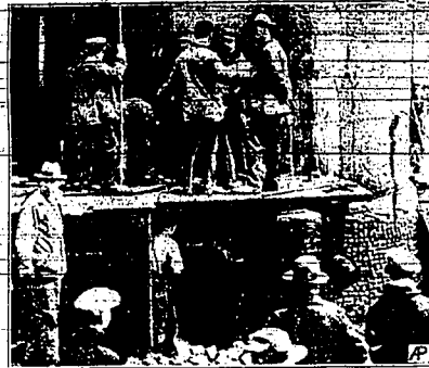
WHEN A SCAFFOLDING on which they were working inside a refuse incinerator collapsed at Everett, Washington, four persons met death and a fifth seriously injured. Photo shows firemen at work after the tragedy.
