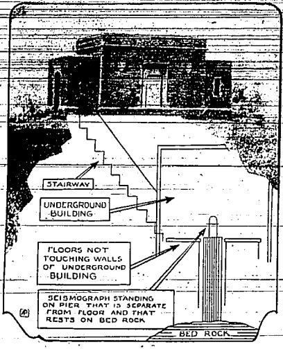
New York City all around it, this Fordham university seismograph station (above) is unaffected by the presence of the metropolis. The instruments are in a separate building resting on bedrock, as shown in drawings.
