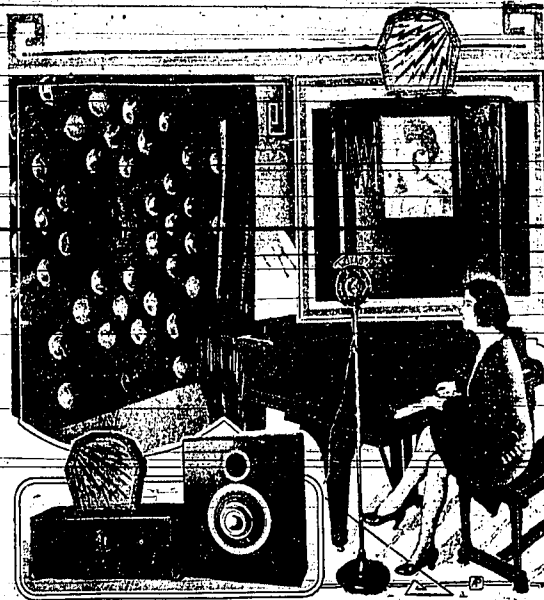
Chicago engineers have synchronized voice and television by using two wavelengths. Helen Rowe is singing and playing before the usual sound microphone, feeding into the WIBO broadcast channel of 525 meters and a television pickup, on 146 meters over W9XAO. Above is a reproducer, with a picture of Yvonne Metz coming in, and below is a smaller television receiver, both designed by the experimenters.
