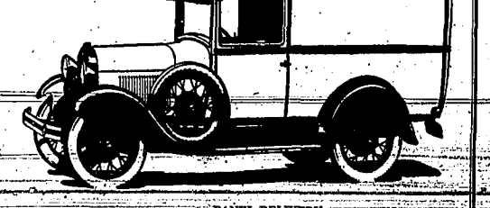
PANEL DELIVERY An attractive model with clean-cut lines. Provides a means of fast, far-reaching delivery service in a vehicle that is good to look at and economical to run. The panel body is built with a wood interior and metal exterior and finished in the standard rock moss green pyralis finish. The roof is covered with heavy-coated rubber material. Large double doors at the rear give a wide opening for quick, easy loading and unloading, and are provided with a handle lock. There is a window in each door. F. O. B. Detroit, plus freight and delivery. Bumpers and spare tire extra.
