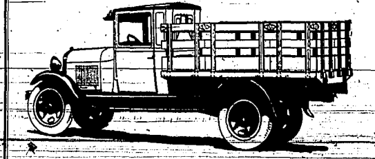
THE FORD 1 1/2-TON TRUCK The chassis of the Ford 1 1/2-ton truck has been materially strengthened at important points. The front axle, front spring and front radius rods are larger and stronger. Service brake drums on the front wheels have been increased to the same size as on the rear wheels, giving far greater braking power and reducing wear on brake linings. F. O. B. Detroit, plus freight and delivery. Bumpers and spare tire extra.
