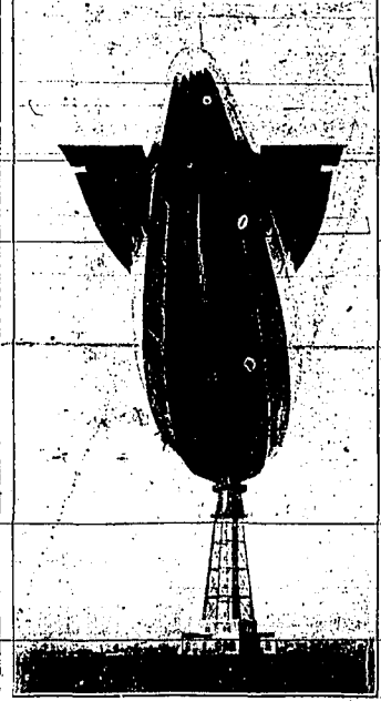
THE BRITISH DIRIGIBLE R-100 moored safely to the new mooring mast at St. Hubert airport, Montreal, after its trans-Atlantic flight from Cardington, England. The dirigible made the 3385-mile trip in 78 hours, despite adverse weather over part of the route and damage to one of its fins. (AP) Photo.
