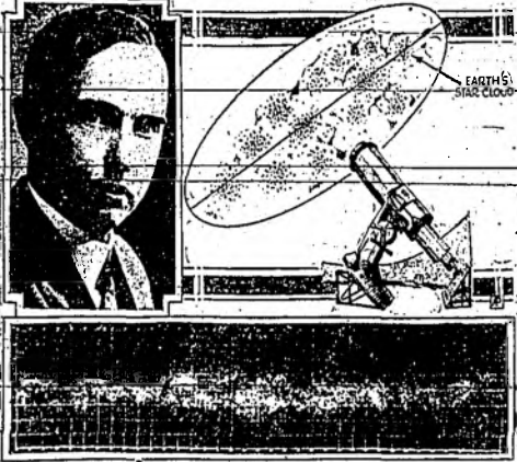
Diagram (top, right) illustrates new theory of Dr. Harlow Shapley (left) of Harvard observatory that Milky Way is not continuous cloud of stars but many separate universes.
