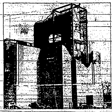
A GIANT 75-TON G-shaped wind tunnel is shown under construction at the Guggenheim airship research institution at Akron, Ohio, where it will be used in testing models of lighter-than-air craft. In the tests huge propellers will drive winds through the tunnel at a velocity of 120 miles an hour.—(P) Photo.
