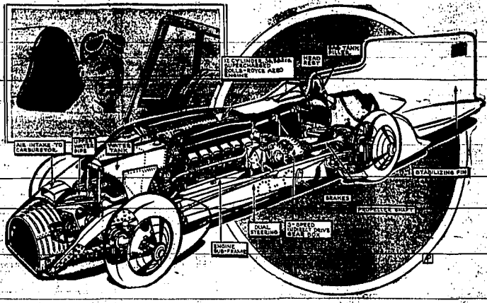
IT TOOK NINE MONTHS of intensive experiment and hard work to piece together this giant racing machine above. The article's drawing gives an inside glimpse of the juggernaut which Six Malcolm Campbell hopes to attain 300 miles an hour at Daytona Beach. The new 12-cylinder engine, in two banks of six cylinders, was so different from the old that it was necessary to remodel the entire front structure.
