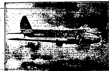
THE NEW bi-motored, 10 passenger transport airplane built in Seattle, Washington, by the Boeing company for the transcontinental run of United Airlines as it looked in flight during a test. It has a top speed of 182 miles an hour and a cruising speed of 166 miles an hour. Several hours will be cut from the running time between San Francisco and New York when this type ship is put in service.—(7) Photo.
