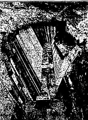
THE NEVADA spillway of Boulder dam is pictured with much of its distance concrete-lined. The proportions of its surroundings disguise the real size of the spillway which is 150 feet wide, 120 feet deep and 650 feet long. Two hundred thousand cubic feet of water can be discharged each second.—(F) Photo.
