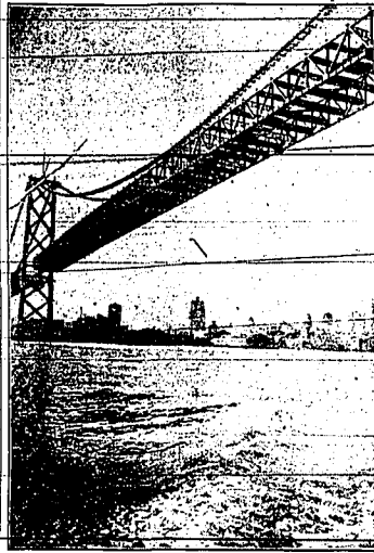
The jutting skyline of San Francisco is picturesquely framed by one of the suspension spans of the giant San Francisco-Oakland bay bridge in this photograph, taken from a boat in mid-bay. It shows the construction progress on the double-deck floor of the bridge being hung from the suspension cables.—(AP) Photo.
