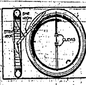
A Lever Taps to Drawing the Rim From Opposite Side So as to Remove the Tire.
