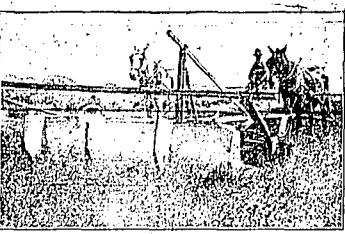
A Combination of Three Small Hopperdozers Attached to Wheels in a Manner to be Pushed by Horses instead of Drawn by Them.
