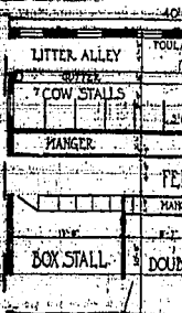
Floor Plan of Small Barn
