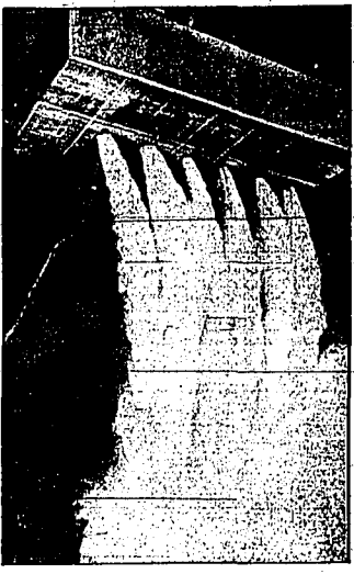
A DOUBLE waterfall 13 feet higher than Niagara will be created today when Boulder dam's outlet valves are tested with the starting of power.
