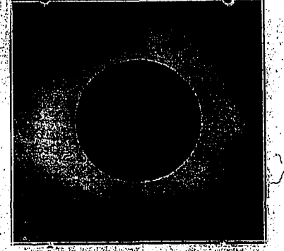
Plumed helmet of the sun's corona taken on June 8, 1918. It is only during the total eclipse that the brilliant corona can be seen. Its beam about two million or even nine million miles from the sun.
