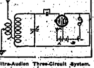
Ultra-Audion Three-Circuit System. condenser, it may be just right before good results are obtained.
