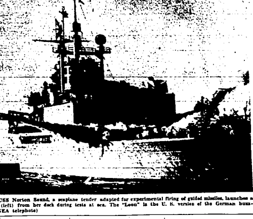
The USS Norton Sound, a seaplane tender adapted for experimental firing of guided missiles, launches a "Loon" (left) from her deck during tests at sea. The "Loon" is the U. S. version of the German buzz-bomb. (NFA telephoto.)
