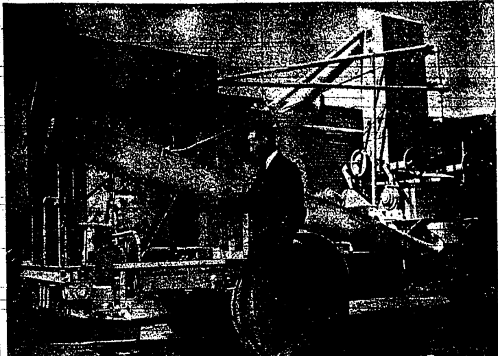
Don Thomas, former Gooding resident, points to the boiler of a portable steam-rolling mill invented by W. J. Southworth, Oakley. It is the second of its kind, Southworth operating the original model near Oakley, Thomas, in partnership with the inventor's son, Mark Southworth.
