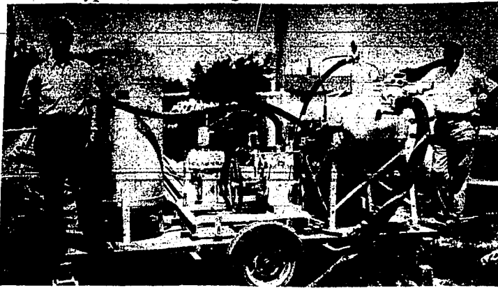
The equipment shown above is a new type of vacuum gold dredge to be used in an attempt to recover gold from mining property near Leesburg in the Salmon district. The machine is the only one of its kind in the world. John Kane of Los Angeles, the co-inventor, is shown at left, Ralph Scheerer, Twin Falls, right, is leasing the equipment. The machine is portable. (Staff photo-engraving.)
