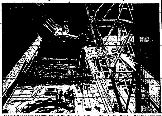
At top left is shown the west face of the dam being built near Bliss by the Morrison-Knudsen company for the Idaho Power company. In the foreground is part of the coffer dam which protects the installation while workers complete construction. On top right the west face of the dam is shown with the steel for the four huge gates which will control the flow of water through the structure. In the foreground is part of a mammoth walking crane which handles heavy machinery. In the center foreground are men working where one of the generators will be installed. Other workers are above of the "pile", an integral part of the installation. At bottom left is the east face of the dam, abutting two of the four gates and in the foreground is the concrete structure of the dam.
