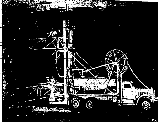
With scores of specially designed machines like the big mobile drill, the U.S. bureau of mines believes it has licked the cost problem which has blocked the way to effective conversion of oil shale rock into usable oil.
