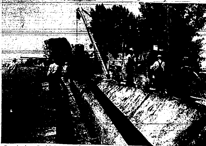
Shown above is a portion of the heavy equipment being used near Burley in pushing a pipeline from Salt Lake City to Boise. In the background is a self-propelled sealing and wrapping machine balanced by a workman holding the pipe at the left. At the right is the "dope" machine which keeps the seal coat at the proper temperature, and is kept burning night and day. Construction crews are making rapid progress on the project and expect to reach Boise by winter. (Staff photo-engraving)
