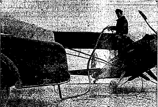
Believed to be the only one of his kind at a municipal field in Idaho, a new gasoline truck (provided by Standard Oil of Calif.) is now in operation at the Twin Falls municipal airport. It is capable of supplying either one or hundreds of gallons of gasoline in planes on any part of the field. Fred Koepnick, Idaho Aviation, Inc. manager, is shown trying it out on one of the small training planes. (Staff photo-enraving)
