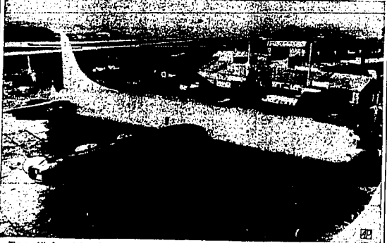
The world's largest land-based cargo plane, the army air force XC-99, stands nearby buildings in the experimental yard of the Consolidated-Vultee plant at San Diego, Calif., where the plane is under construction. It is designed to carry 400 troops or 100,000 pounds of cargo. (AP wirephoto from AAF.)
