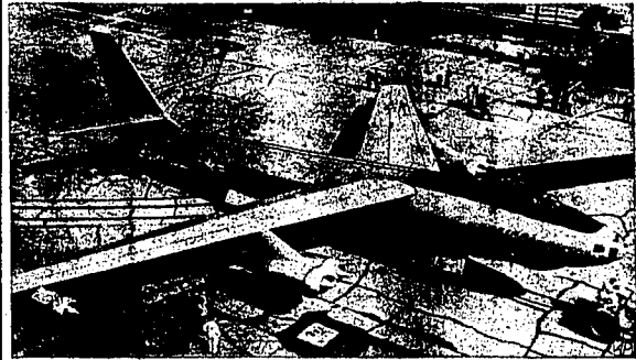
As large as a B-29 Superfortress, this new Boeing XB-47 rolled out of hangar in Seattle, Wash., in powered with jet engines. The army air force and Boeing call it a "radical new experimental design" with the inverted wings and tail surfaces. Ground and taxing tests start soon. (AP wirephoto)
