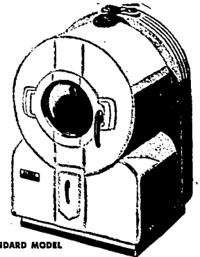
STANDARD MODEL
