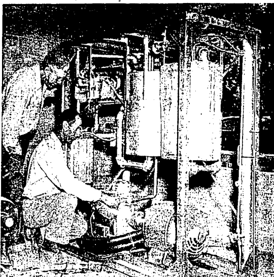
Common well water processed by the 'heat pump' pictured above can provide the source of both heat and cooling in buildings where it is installed. Harold Minnety and Frank McClear are shown inspecting the machine installed at a new coffee shop. (Staff photo-enlarging)
