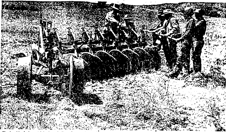
The brushland plow, at left above, is the only one of its kind in existence. It can be used in heavy brushland and on rocky ground. The discs are indelibly sprung so the machine may be used over rocks without damage.
