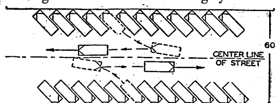
CAPACITY OF STREET WITH ANGLE PARKING IS APPROXIMATELY 600 VEHICLES PER HOUR
