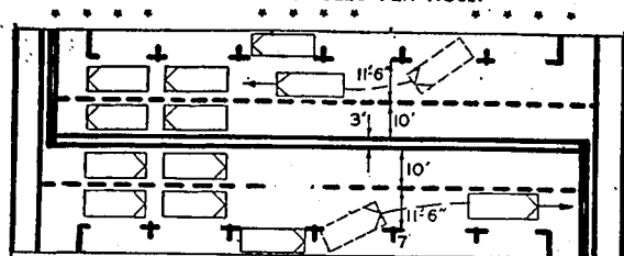
CAPACITY WITH PARALLEL PARKING IS 1500 TO 1800 VEHICLES PER HOUR
