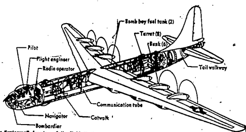
This "cutaway" drawing of the B-36, U. S. air force super bomber, is the first to be released by Consolidated Vultures and the air force. The sketch shows general arrangement of the plane's 102-foot-long fuselage against fighters are viable. In addition to the six standard engines, late models of the B-36 are being equipped with four jet engines.
