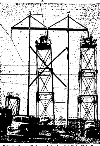
Here are three mobile towers designed and built by Idaho Power company personnel to speed construction of a transmission line between Bliss and American Falls. The line started operation Tuesday night. Two of the towers are elevated to full height with men working on lines. The third tower is lowered for traveling to the next pole.
