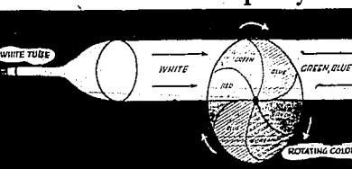
This diagram shows the basic elements in a television set used to receive a color television picture. CBS "field sequential" system.
