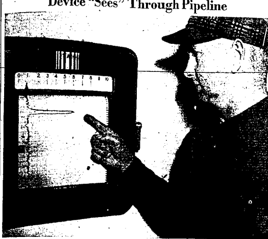
Russell Spencer, stock delivery man at the Salt Lake Pipe Line company take-off point southwest of Twin Falls, points to a recorder connected with an electronic device attached to the line to detect chemical markers between various products delivered in the line. When the chemical marker passes by the electronic device the recorder sends a signal across the chart as shown above. Two sets of the instruments are used, one further up the line to give advance notice. (Staff photo-entwain)
