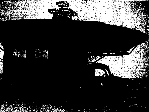
Equipment in this strange-looking truck is used to broadcast navigation signals at Joslin field in tests preliminary to probable installation of new navigation equipment at the Twin Falls airport. The truck unit is called a portable omnirange navigon ground unit.
