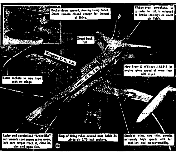
Photo-diagram above shows outstanding features of the radically new Lockheed P-94 Starfighter, now in production at Burbank, Calif., and being delivered to the air force. The Starfighter carries no guns, relying on rockets. It is a nearly automatic that the pilot and radar operator have little else to do but take the plane off the ground, maneuver to the general target area guided by ground radar, switch on the "electronic crew" monitor operation of the plating and rocket-control apparatus during the attack and then land. The all-weather interceptor is designed for air defense of the United States, with the specific mission of knocking out enemy bombers.
