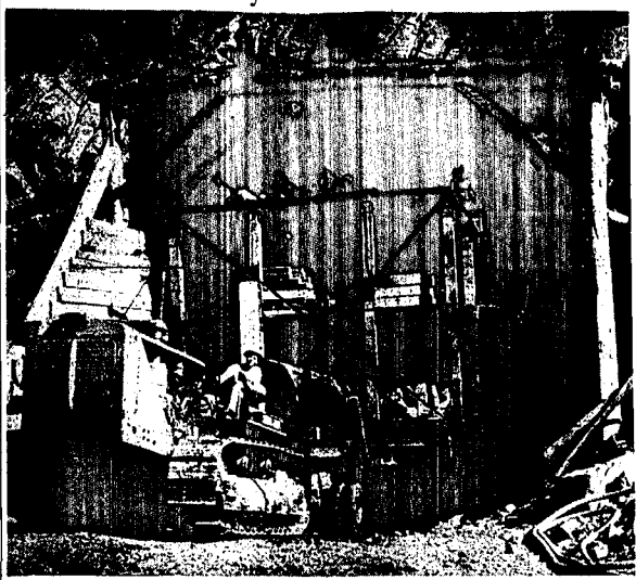
A triple-decker "jumbo" drill rig is at work driving two 31-foot diameter diversion tunnels through the rock abutment of Palisades dam. Mounted on the decks are 15 compressed air drills which are drilling holes 8 to 12 feet deep. After drilling about 120 holes, the "jumbo" is wheeled out by the tractor and the holes are loaded and blasted. While the loose material is being removed from one of the tunnels, the jumbo goes to work on the other. Both tunnels will be concrete-lined to an inside diameter of 25 feet. Later, one will become a power tunnel, 1,215 feet long, and the other an outlet tunnel, 1,550 feet long.
