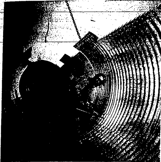
This circular pipe, seven feet in diameter and 500 feet long, is required for drainage under a big road fill near Fallsdam dam, now being constructed on Snake river in eastern Idaho. The road fill, known as the Big Elk creek fill, will be the largest in Idaho, involving placement of a million and one-half cubic yards of material. It is a phase of the job of relocating U. S. Highway 20 around a part of the 1,600-acre-look, 20-mile-long reservoir which the dam will create. (Bureau of reclamation photo—staff engraving)
