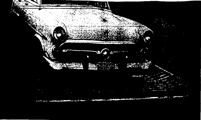
This cattle-guard devised by an irrigation district manager in eastern Oregon permits cars to pass without the bother of opening gates, yet it stops cattle. The low-cost, portable guard can be constructed in home shops. (Bureau of reclamation photo—staff engraving)
