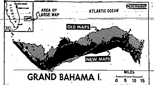
Misguided map for guided missiles. Solid black portion of map is the way Grand Bahama Island, off Florida, is actually located as proven by shore and triangulation surveys in 1931. Shaded area is the way Bahama had been charted up to then, with the shoreline as such as seven miles in error. Small map shows relation of Bahama to Florida missile range in Florida.
