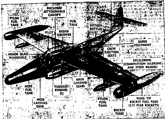
This phantom view discloses internal details of America's most heavily armed fighter plane, the USAF's Northrop Scorpion F-89D. Details are shown of the deadly wing-tip rocket-fuel pods. Their ingenious design permits rockets to be carried in the fore part of the pod and fuel in the rear portion. Also new is the long-range nose fuel tank, which was not carried on the earlier F-89C model. The plane is armed with 104 2.75-inch folding-fin, air-to-air rockets. Advanced electronic aiming and automatic triggering enables the Scorpion's two-man crew to seek out invading aircraft regardless of darkness or bad weather. (NEA)
