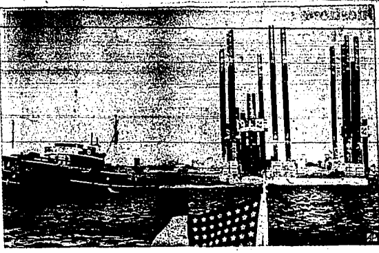
Tugs tow the Texas tower radar station down Boston, Mass., harbor en route to its destination on Georges Banks, 118 miles east of Cape Cod. The 2,900-ton steel structure will become a man-made island and America's first offshore radar outpost. When the tower reaches its destination its three legs will be sent down to the ocean bottom, 50 feet below the surface; their drivers 45 feet more into the earth. The triangular platform will be lifted 68 feet above the surface of the sea by the giant legs. (AP wirephoto)
