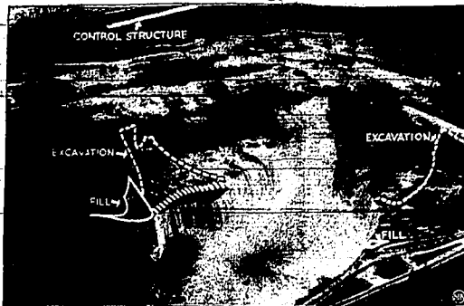
Diagrammed photo shows the work now under way at Niagara Falls to beautify this major tourist attraction. Near top is the excavation of the 13 slopes that will form the control structure, while on both flanks are excavation and fill work to be done by I.W. (W.M.A. photo).
