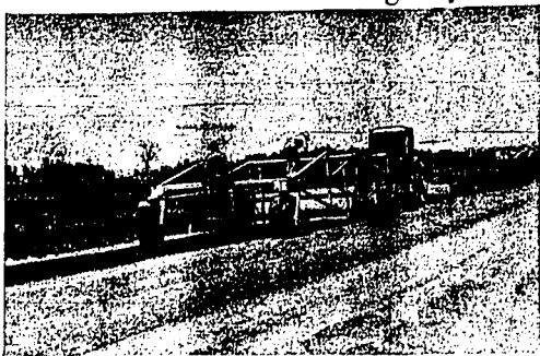
The land plane shown above is being used as an experiment on the Beeches Corner-Ririe road. The leveler was used with success on the surface course. A smoother riding surface was provided on six sections where the land plane was used than on the two sections leveled by ordinary methods. As far as is known, this is the first time a land plane has been used on highway construction.
