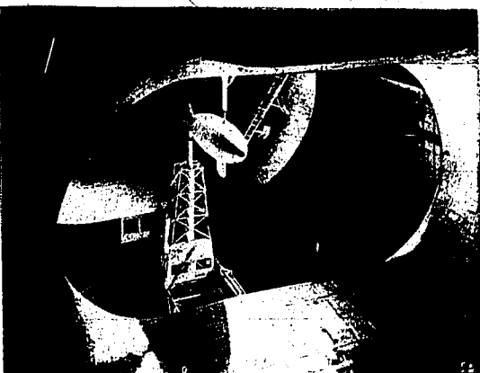
A one-fifth scale model of the submarine Albacore hangs in a wind tunnel at the national advisory committee for aeronautics at Langley Field, Va. NACA scientists conducted this unusual experiment to help the navy improve hull contour. The navy announced its future atomic and conventional-powered subs will have the same shape as the Albacore, reputed to be the world's fastest submarine. (AP wirephoto)
