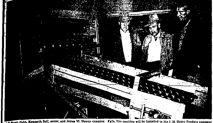
The first production model of a standard six-channel potato stamping machine assembled at the Self Manufacturing company plant in Twin Falls. The machine will be installed in the J. H. Henry Produce company potato warehouse in Kimberly. Self plans to produce more than 200 of the marking machines this year for Idaho. (Staff photo-engraving)
