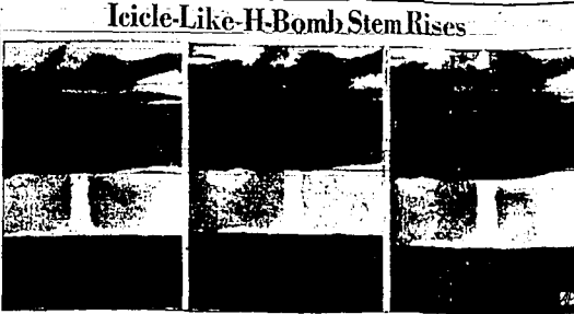
Ice-icle-Like H-Bomb Stem Rises An ice-icle-like stem pierces dark cloud and extends skyward following the explosion of a hydrogen bomb over tiny Namu Island in the Bikini atoll in the Pacific. It was the first H-bomb to be dropped from a U. S. aircraft. These pictures were made with a sequence camera from aboard the observer ship USS Mt. McKinley about 36 miles from the blast site. No indication of time lapse following the explosion was indicated to caption material accompanying the pictures. (AP wirephoto)
