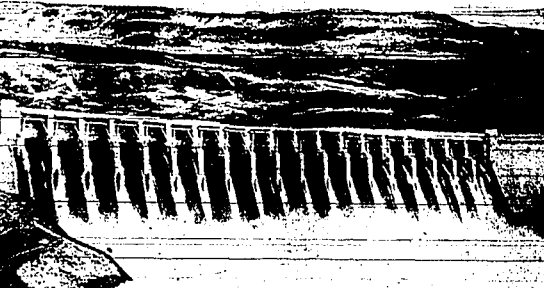
Muddy Columbia river water pours through gates of the 4,200-foot-long, 230-foot-high Chief Joseph dam, a gigantic hydroelectric power project which was officially dedicated by Presidential Assistant Harold Stassen at Bridgeport, Wash. Located below Grand Coulee dam, the Chief Joseph project becomes the second largest electric power generating unit on the Columbia river drainage. (AP wirephoto)
