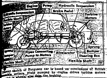
Carry sketch of Ferguson car is based on conclusions of British writers. Fluid pumped by engine drives turbine motors to wheels, also does the braking.
