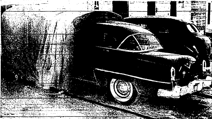
Don Teeter's canvas and metal-frame garage can be compressed to a length of three feet for easy access. Once the car is in position, the garage is closed by pulling on the cable shown lying on the ground at the foot of the garage. The metal frame slides forward on rollers which the inventor has devised.
